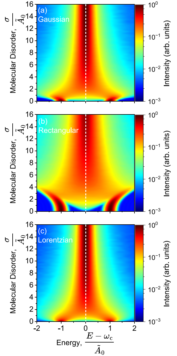
FIG. 7. Transmission spectra for N = 100 at varying Gaussian energetic disorders (vertical axis) of the molecules with widths \sigma with distribution (a) Gaussian, (b) rectangular, and (c) Lorentzian. A_0 = 0.01 a.u., \omega_c = 1.00 a.u., N_r = 50\,000 , N_{\text{Cheb}} = 2500 , \gamma = 0.001 a.u. Note that the data shown here are identical to Fig. 6 except that the intensity is on a log scale.
