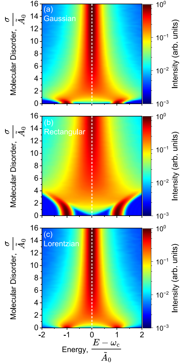
FIG. 9. Transmission spectra for N = 1000 at varying Gaussian energetic disorders (vertical axis) of the molecules with widths \sigma with distribution (a) Gaussian, (b) rectangular, and (c) Lorentzian. A_0 = 0.01 a.u., \omega_c = 1.00 a.u., N_r = 50\,000 , N_{\text{Cheb}} = 2500 , \gamma = 0.001 a.u. Note that the data shown here are identical to Fig. 8 except that the intensity is on a log scale.
