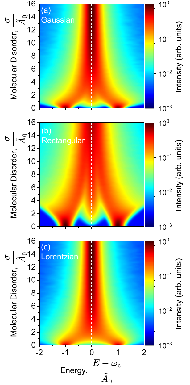
FIG. 5. Transmission spectra for N = 2 at varying Gaussian energetic disorders (vertical axis) of the molecules with widths \sigma with distribution (a) Gaussian, (b) rectangular, and (c) Lorentzian. A_0 = 0.01 a.u., \omega_c = 1.00 a.u., N_r = 50\,000 , N_{\text{Cheb}} = 2500 , \gamma = 0.001 a.u. Note that the data shown here are identical to Fig. 4 except that the intensity is on a log scale.
