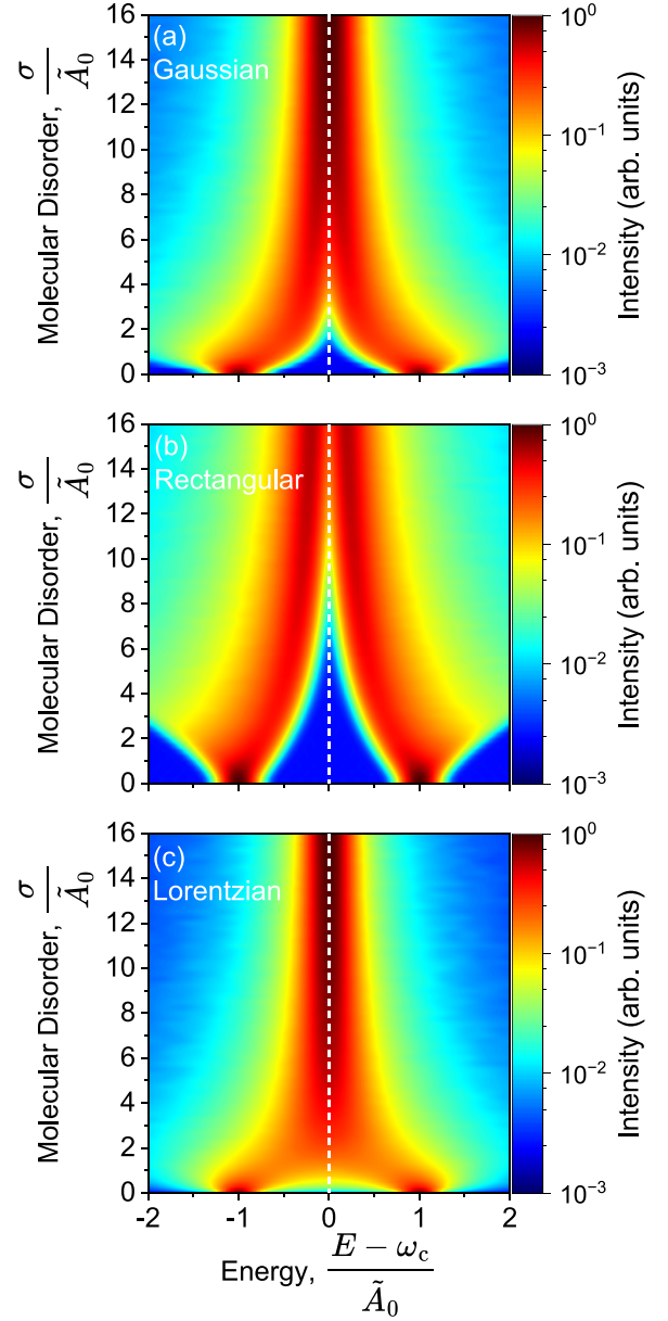
FIG. 3. Transmission spectra for N = 1 at varying Gaussian energetic disorders (vertical axis) of the molecules with widths \sigma with distribution (a) Gaussian, (b) rectangular, and (c) Lorentzian. A_0 = 0.01 a.u., \omega_c = 1.00 a.u., N_r = 50\,000 , N_{\text{Cheb}} = 2500 , \gamma = 0.001 a.u. Note that the data shown here are identical to Fig. 2 except that the intensity is on a log scale.
