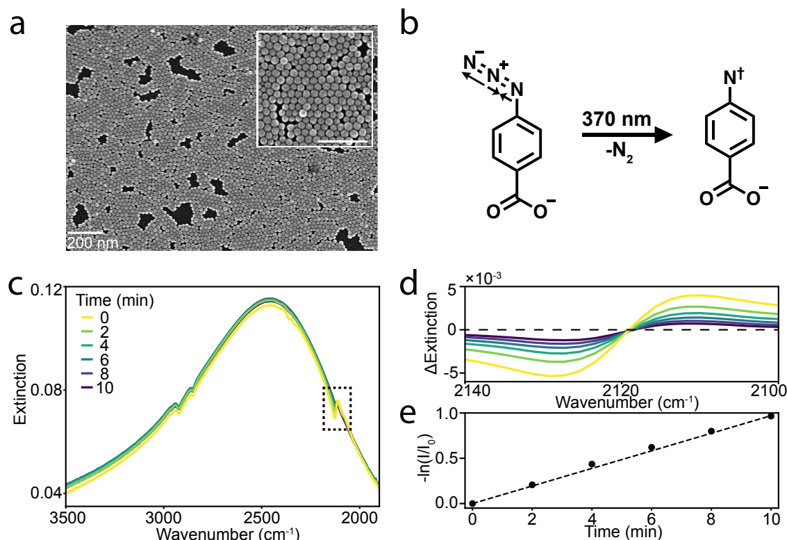
Figure 1: ITO NC monolayer used for kinetic control over 4-azidobenzoic acid (ABzA) photolysis. (a) Top-down SEM image of a 0.9% Sn doped ITO NC monolayer, where native oleate ligands have been exchanged with ABzA molecules. The inset shows the NC film at high magnification, with the scale bar indicating 200 nm. (b) Photolysis of ABzA following illumination with 370 nm light, resulting in loss of N_2 and forming a reactive intermediate. Arrows on the reactant molecule highlight the asymmetric stretching mode of the azide group, which is lost after the reaction proceeds and is monitored to quantify reaction progress. (c) Time-evolution of the extinction spectra of a 2% Sn doped ITO NC monolayer under illumination from a 370 nm light-emitting diode (LED), highlighting the asymmetric azide stretching mode. (d) The asymmetric (Fano lineshape) azide stretching mode decays as a function of UV illumination time after subtraction of the CPR background using polynomial fitting. We recorded the difference between the maximum and minimum of the vibrational signal at each time point. (e) The vibration intensity was normalized to its initial value, and the negative logarithm was taken, resulting in a linear progression as a function of time, indicating the first order kinetic process.
