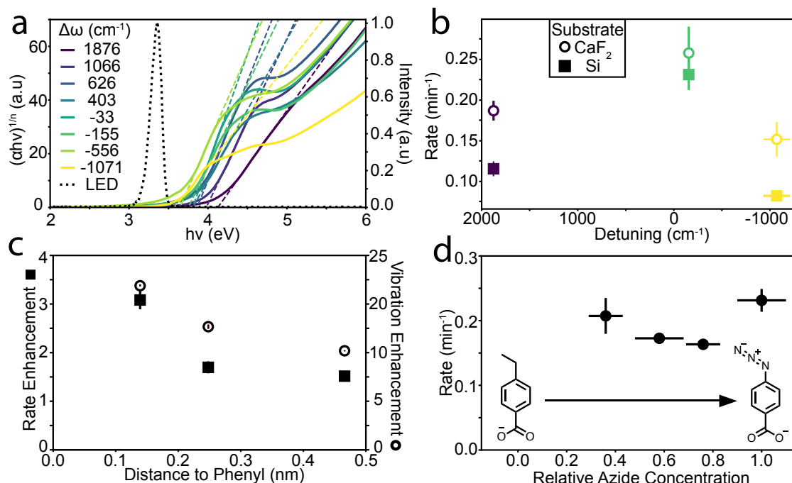
Figure 3: Control experiments to demonstrate that the vibration-CPR resonance drives the enhanced photolysis rate. (a) Tauc plots derived from UV–Vis extinction spectra of ITO NC monolayers, showing monotonically increasing band gap at higher Sn doping concentration. The LED emission profile is overlaid as a dotted black line. Optical band gaps (Table S4), were determined by extrapolating the linear region of the curve to the x-axis (dotted lines). (b) Differences in reaction rates for ITO NCs with varying \Delta\omega , for assemblies deposited on Si (filled squares, select data points from Figure 2e) and CaF 2 (open circles) substrates. (c) Vibrational intensity (open circles) and rate enhancement (closed squares) relative to the same molecule on In 2 O 3 NCs as a function of the length of the molecule from the NC surface to the phenyl ring. (d) Reaction rates in NC monolayers with \Delta\omega = -155 cm -1 at various ABzA concentrations on the NC surface. A mixture of ABzA and 4-ethylbenzoic acid was used to control the relative surface density of azide functional molecules.
